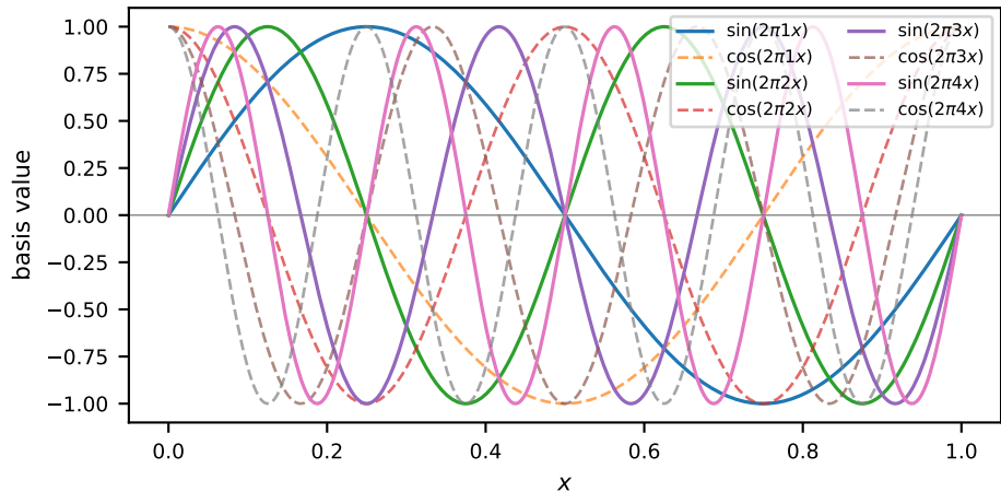
Sinusoidal Basis Functions (Fourier)
