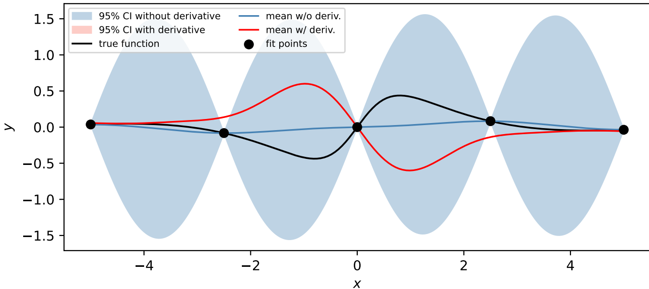
Ex. 18.3: f(x) = \sin(x)/(x^2 + 1) with/without derivative info
