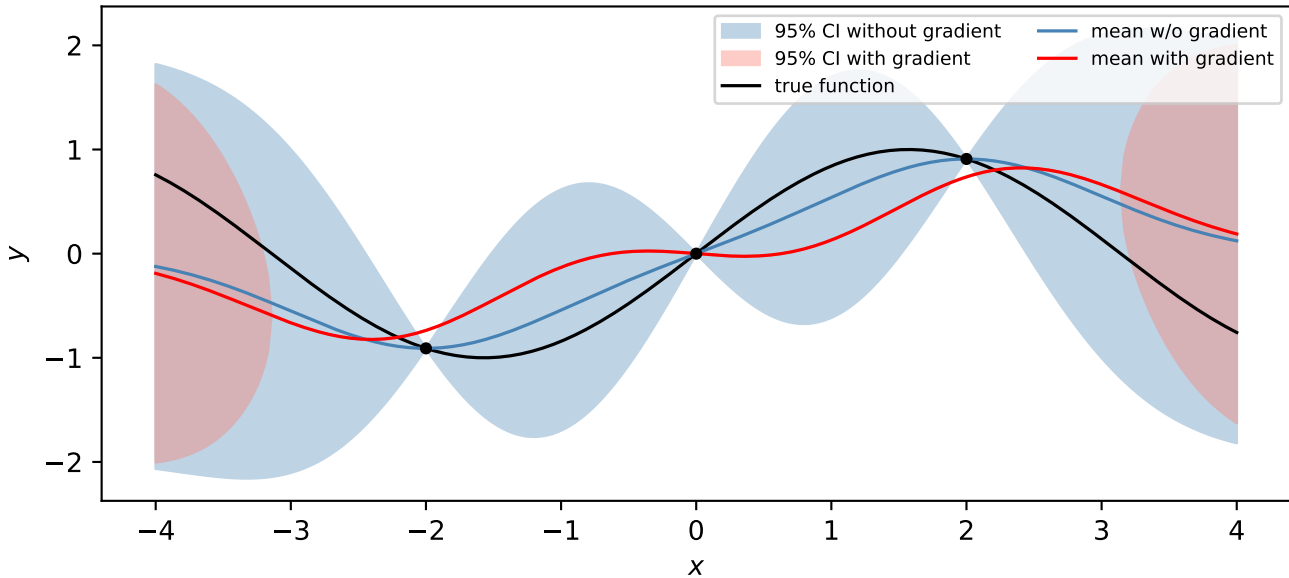
GP with and without Gradient Observations
