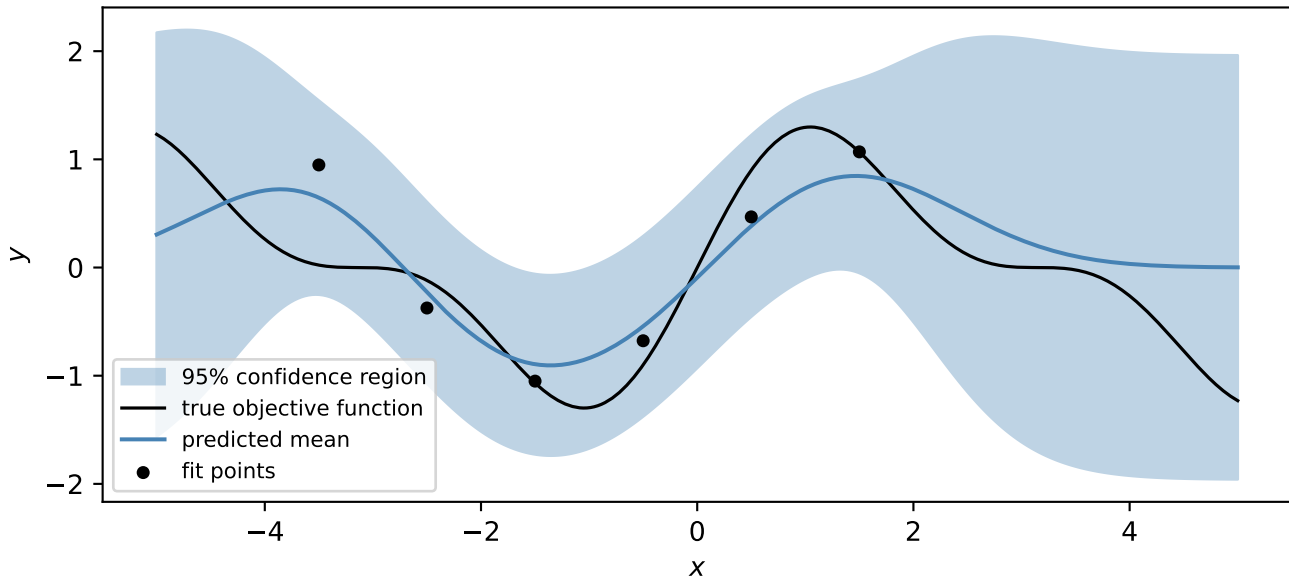
Noisy GP with Squared Exponential Kernel
