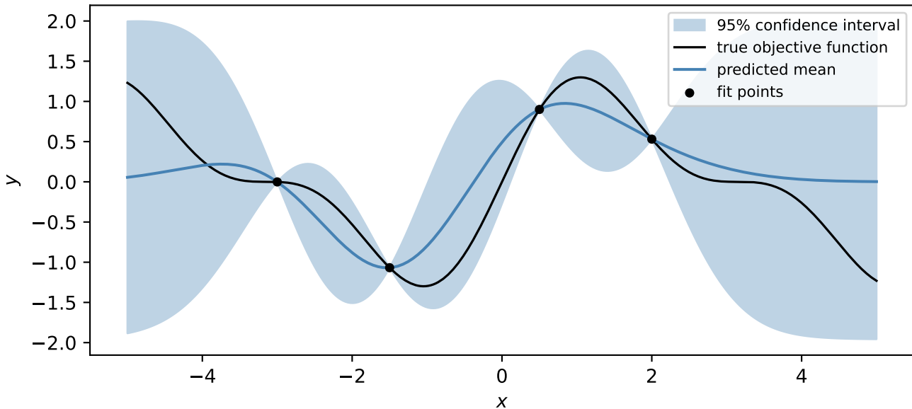
GP with Squared Exponential Kernel (noise-free)
