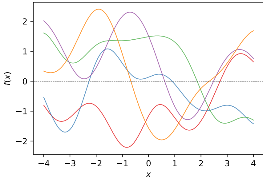
GP Prior Samples (Squared Exp Kernel)
