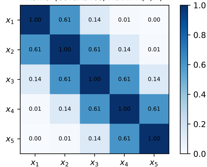
Kernel (Covariance) Matrix K(X, X)
