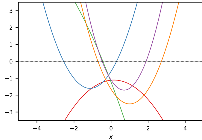
Polynomial: (x^T x' + c_p^2)^p
