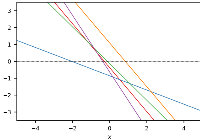
Linear: \sum c_d^2 x_d x'_d
