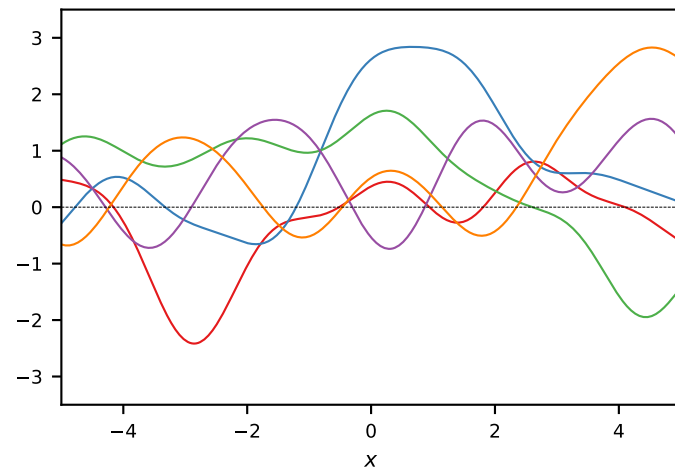
Squared Exp: \exp(-r^2/2\ell^2)
