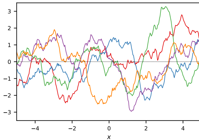
\gamma -Exp: \exp(-(r/\ell)^\gamma)
