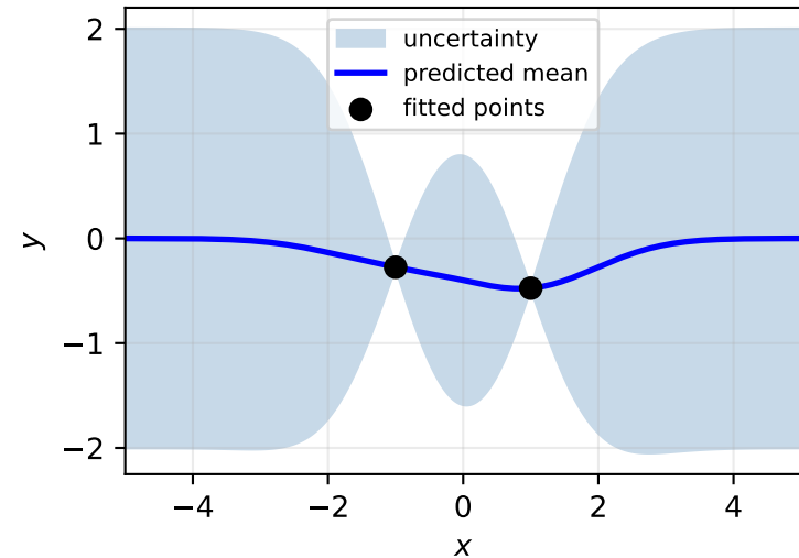
Gaussian Process
