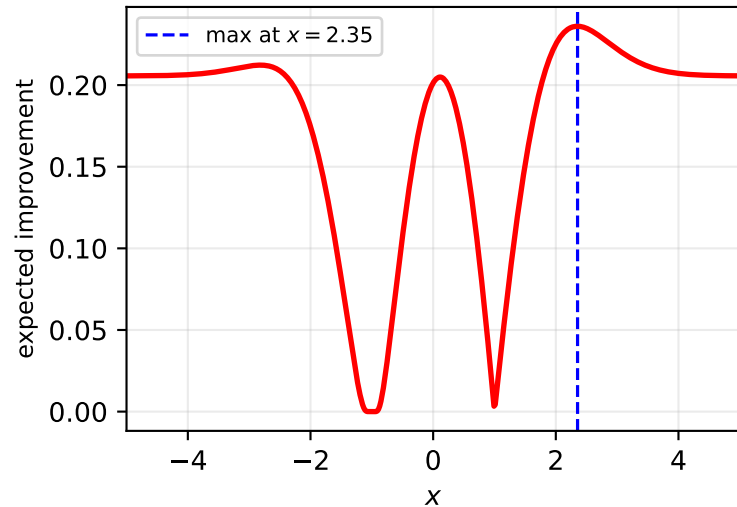
Expected Improvement
