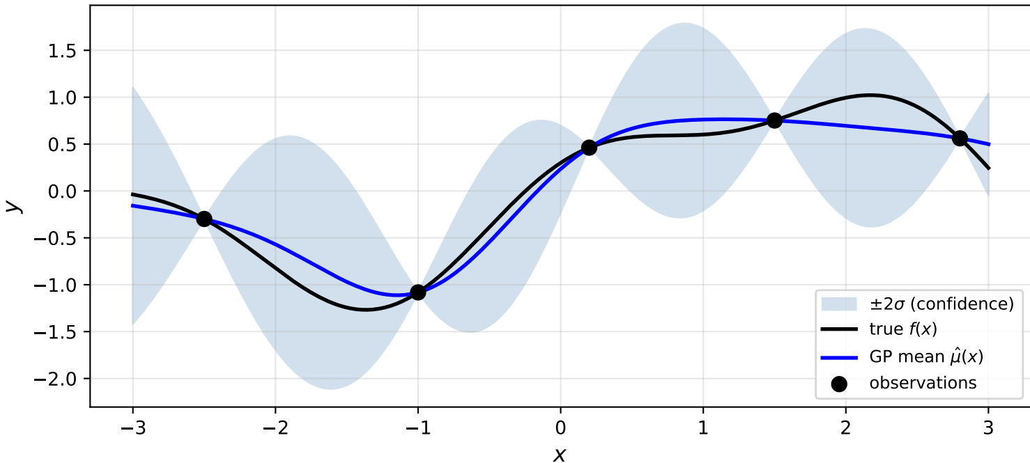
Gaussian Process Surrogate Model
