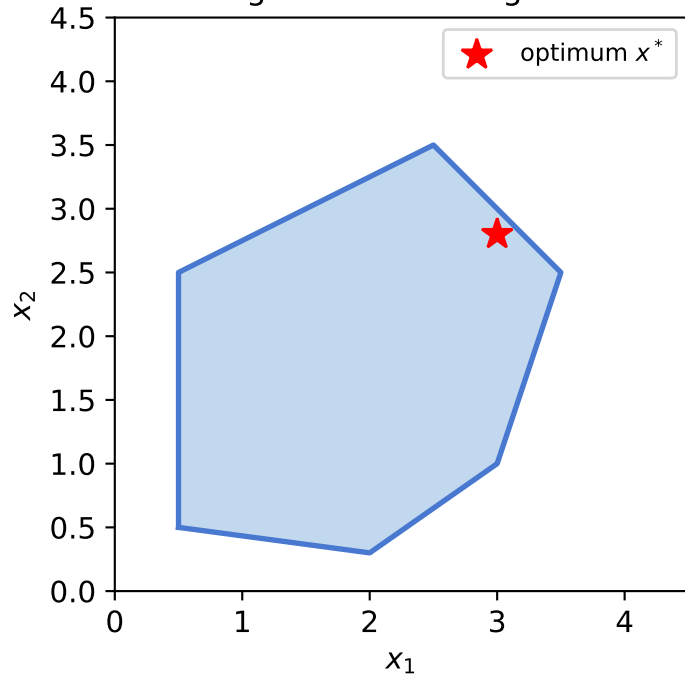
Original feasible region \mathcal{X}
