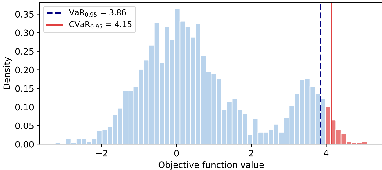
Value at Risk (VaR) vs Conditional Value at Risk (CVaR), \alpha = 0.95
