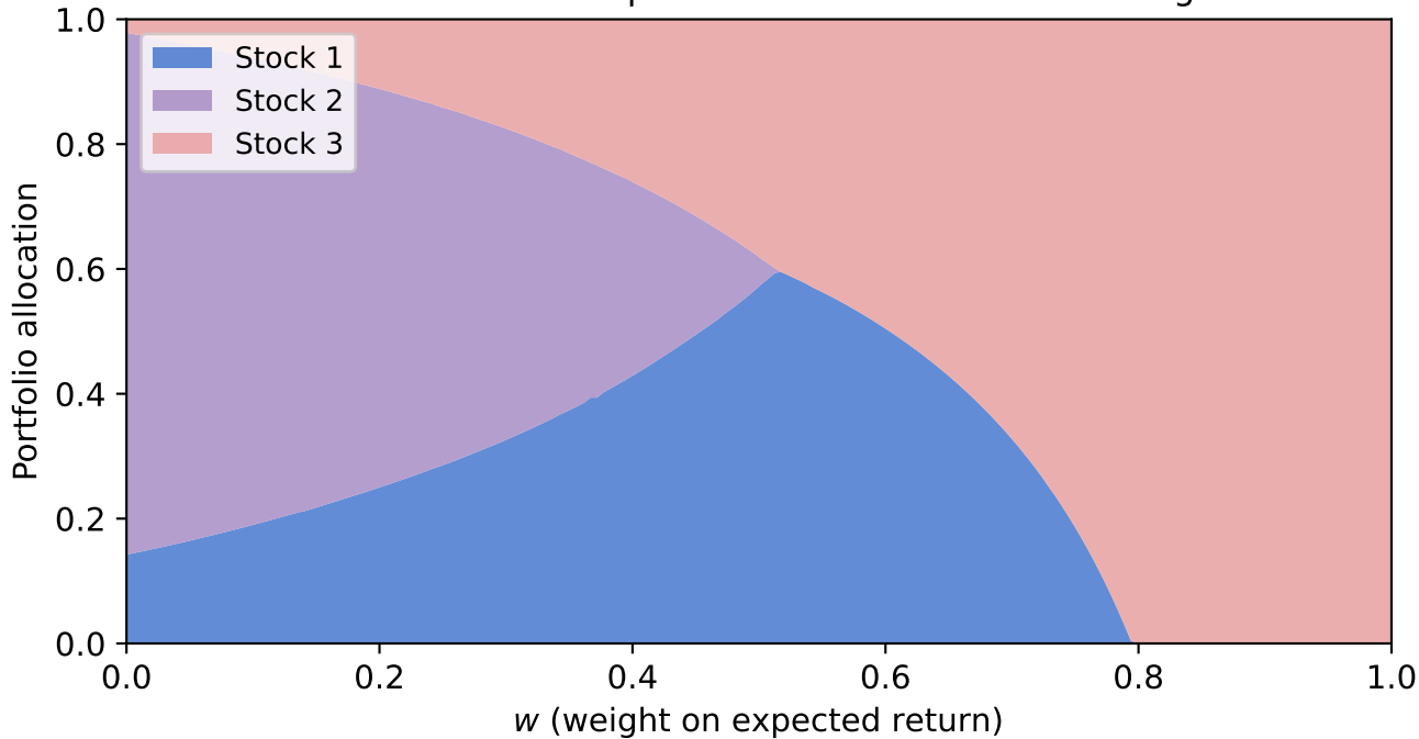
Markowitz Portfolio: optimal allocation vs. return weight w
