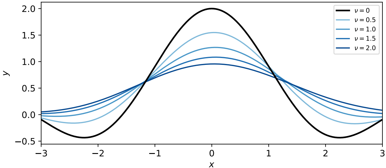
Expected value of f(\tilde{x}) = \sin(2\tilde{x})/\tilde{x} under Gaussian noise
