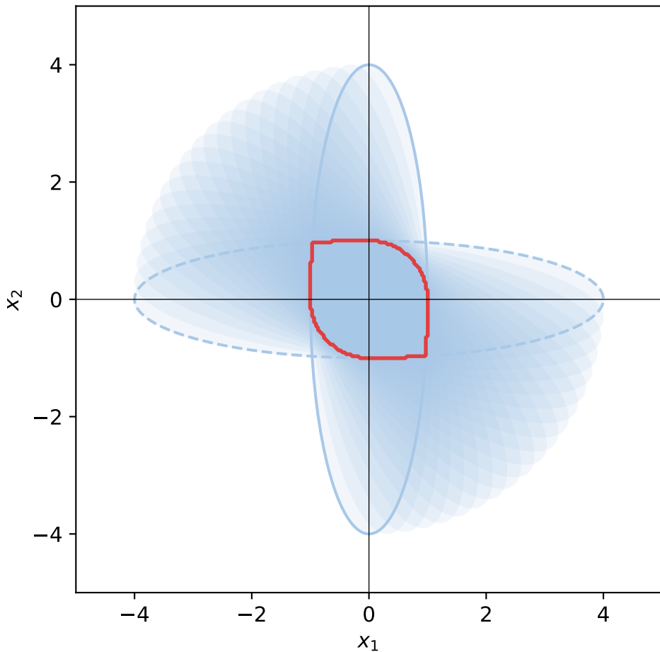
Rotated ellipse feasible sets (blue=union, red=intersection/robust)
