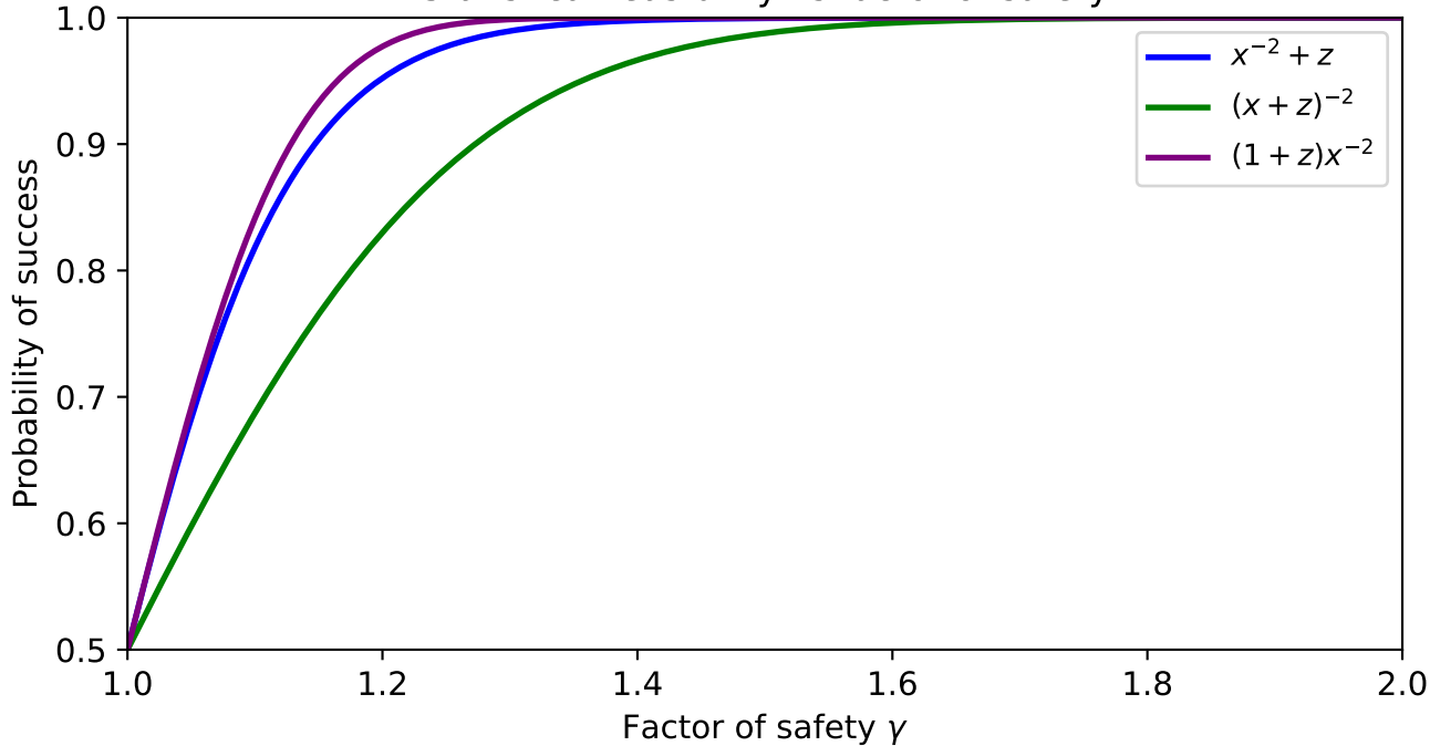
Statistical feasibility vs factor of safety
