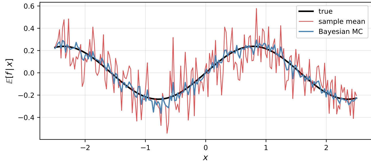
Bayesian MC vs Sample Mean ( m = 10 per point)
