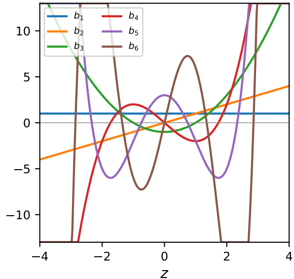
Hermite
