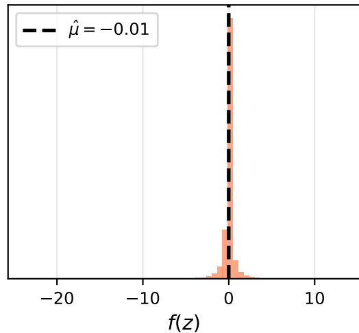
Output distribution
