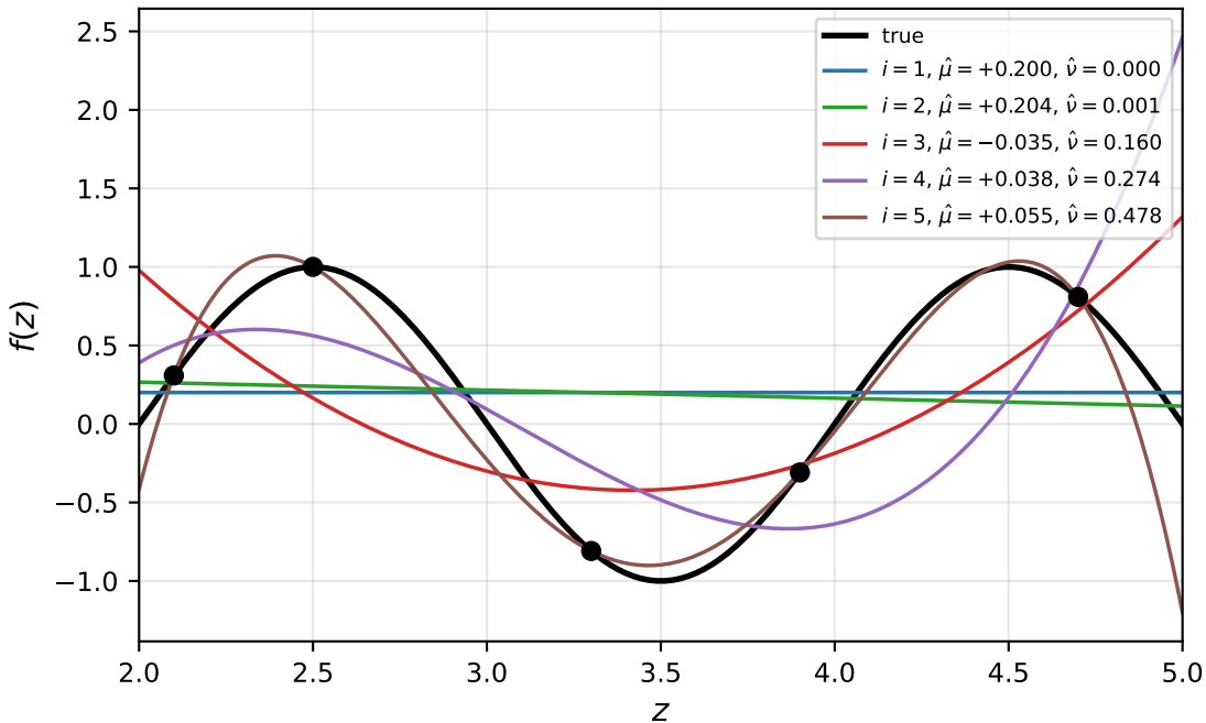
Stieltjes Fit: f(z) = \sin(\pi z) , Truncated Gaussian [2,5]
