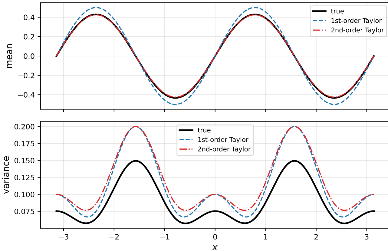
Taylor Approx: f(x, z) = \sin(x + z_1)\cos(x + z_2)
