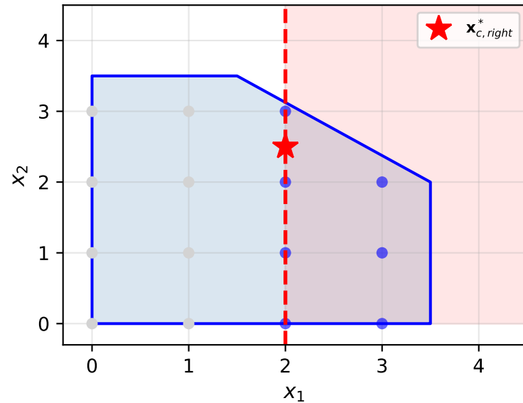
Branch: x_1 \geq 2
