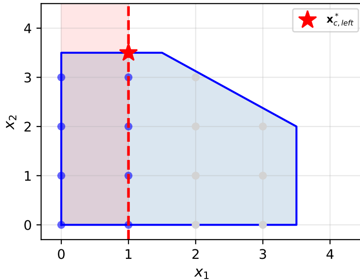
Branch: x_1 \leq 1
