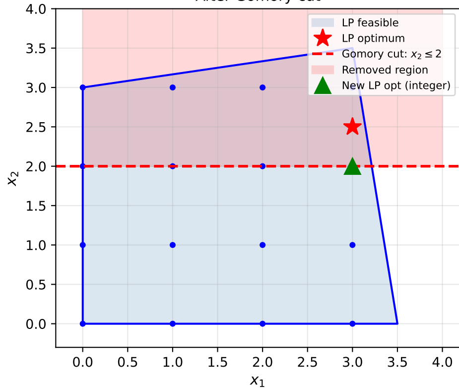
After Gomory cut
