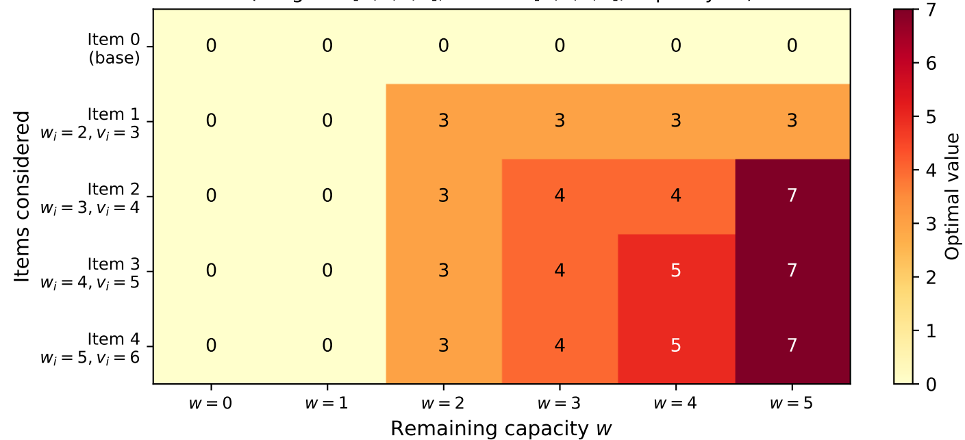
0-1 Knapsack DP Table (weights=[2,3,4,5], values=[3,4,5,6], capacity=5)
