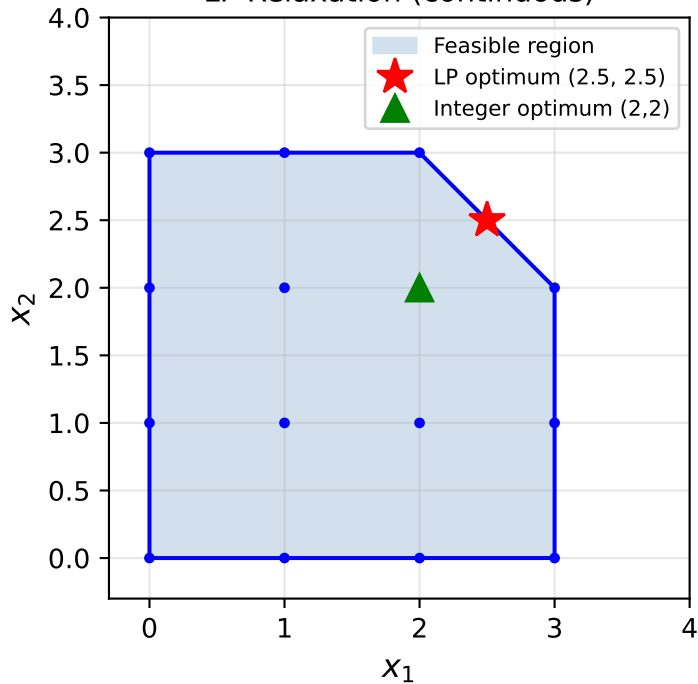
LP Relaxation (continuous)
