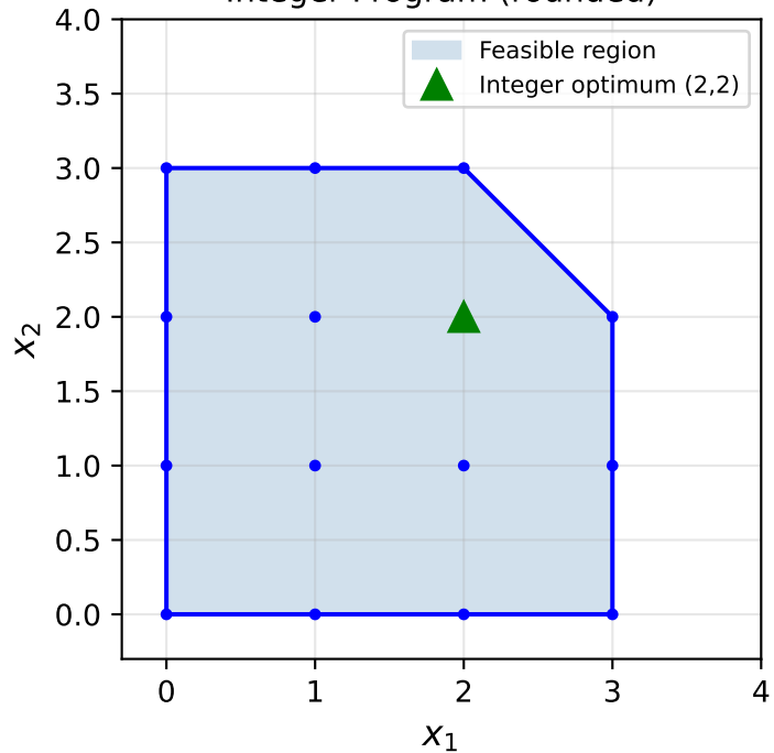
Integer Program (rounded)
