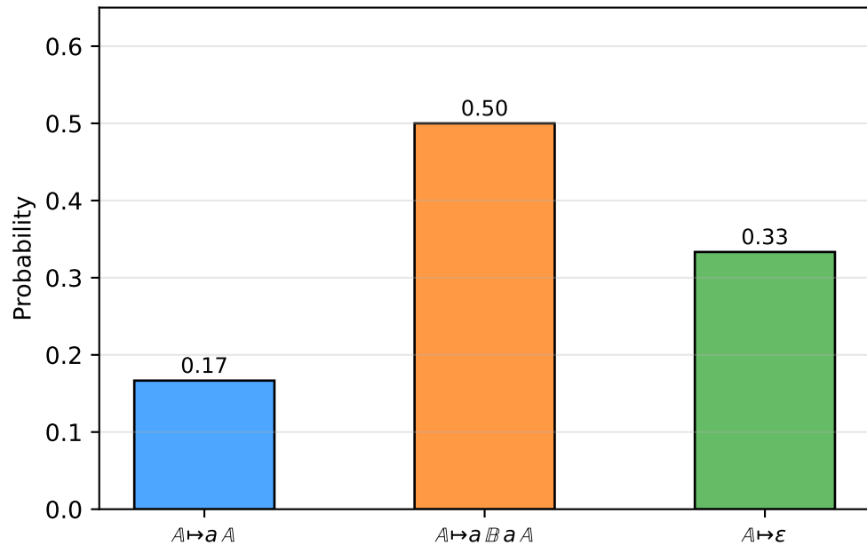
Production Probabilities for type A
