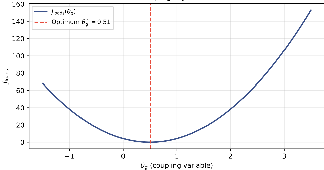
CO Subproblem: Coupling Objective vs. Global Variable
