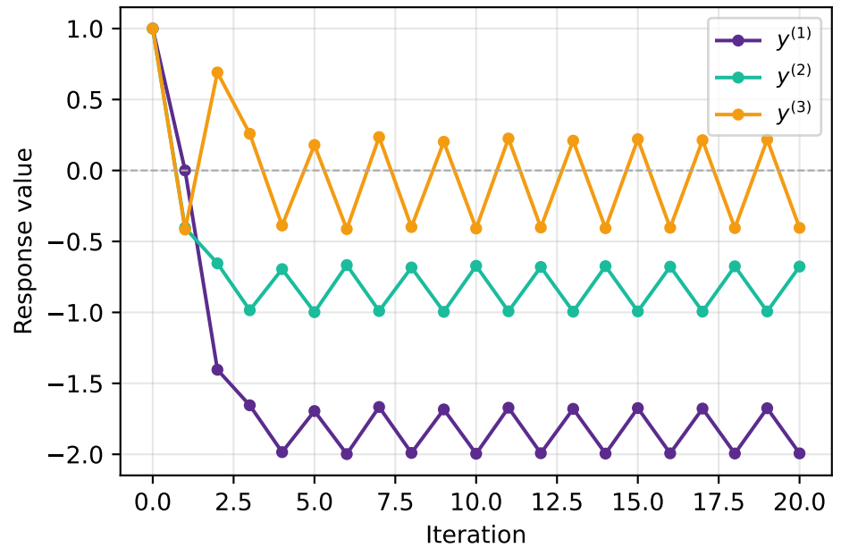
Ordering F_1, F_3, F_2 (diverges)
