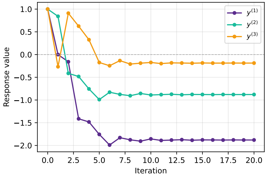
Ordering F_1, F_2, F_3 (converges)
