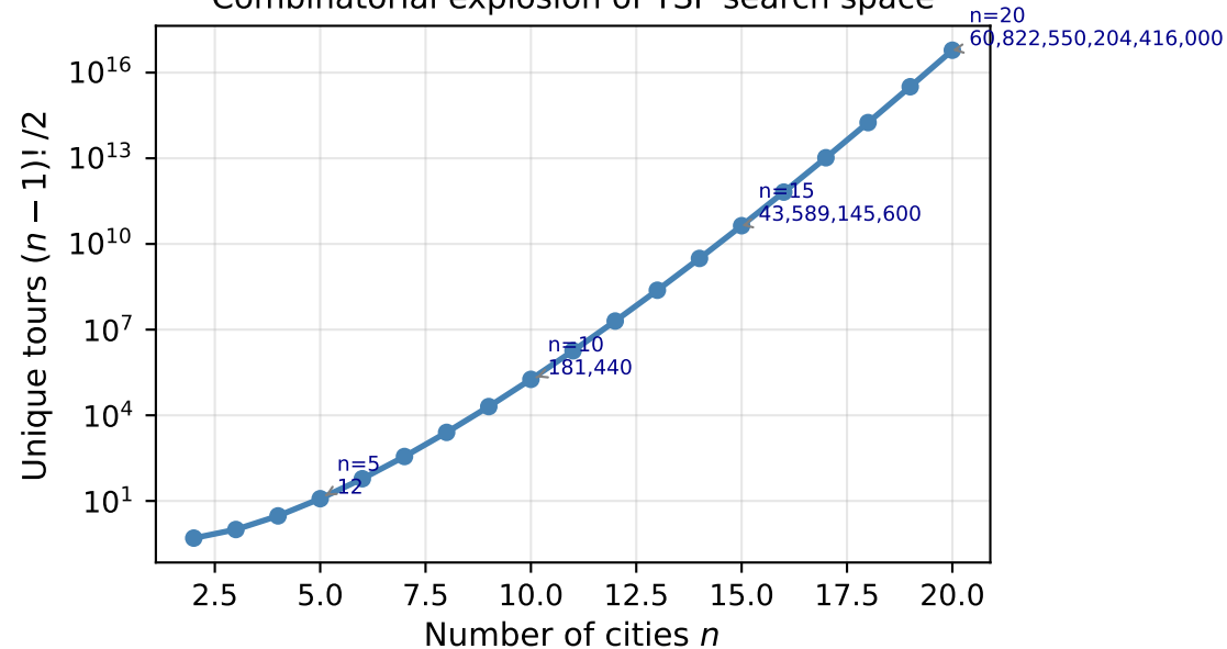
Combinatorial explosion of TSP search space
