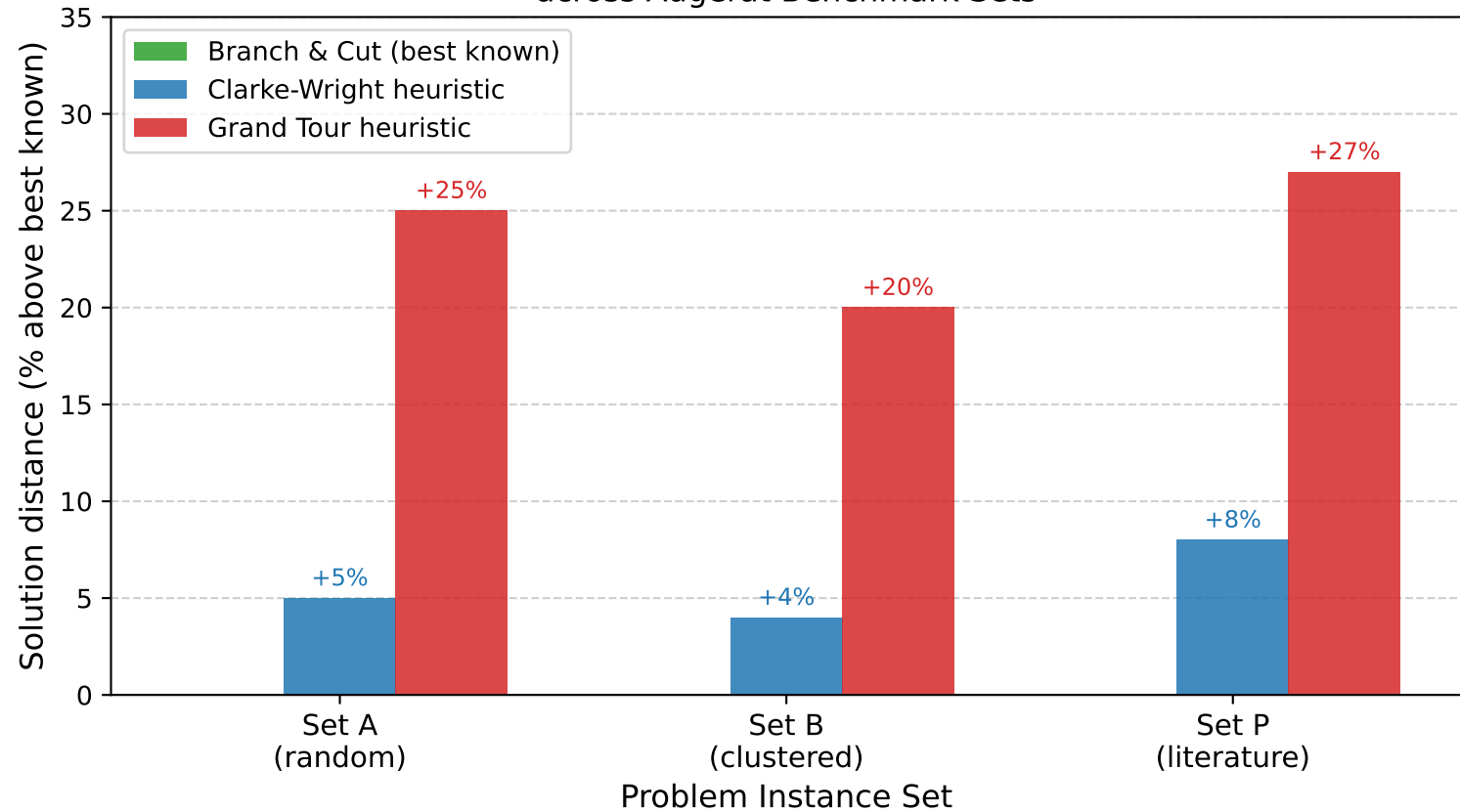
Algorithm Performance Comparison across Augerat Benchmark Sets
