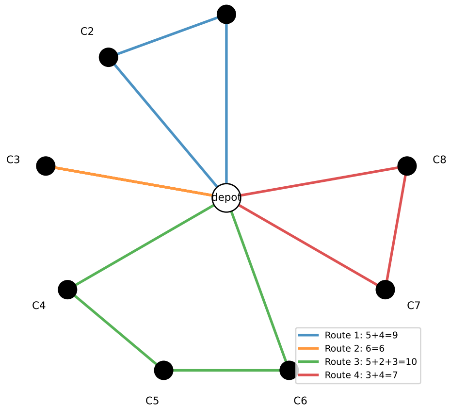
Split into Sub-tours (capacity = 10)
