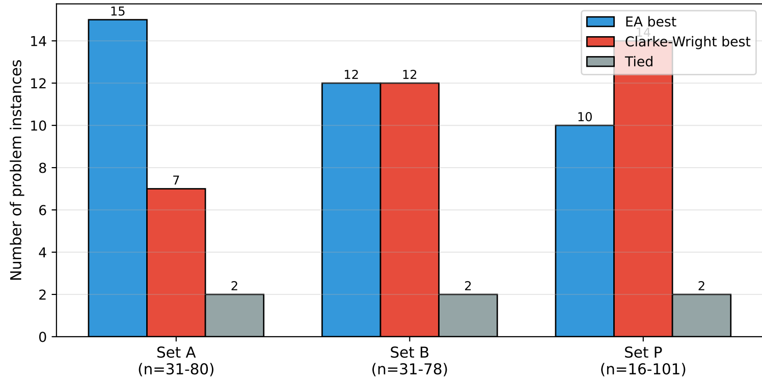
EA vs Clarke-Wright: Best Solution per Instance (Augerat 1995 benchmark; EA is competitive on smaller instances)
