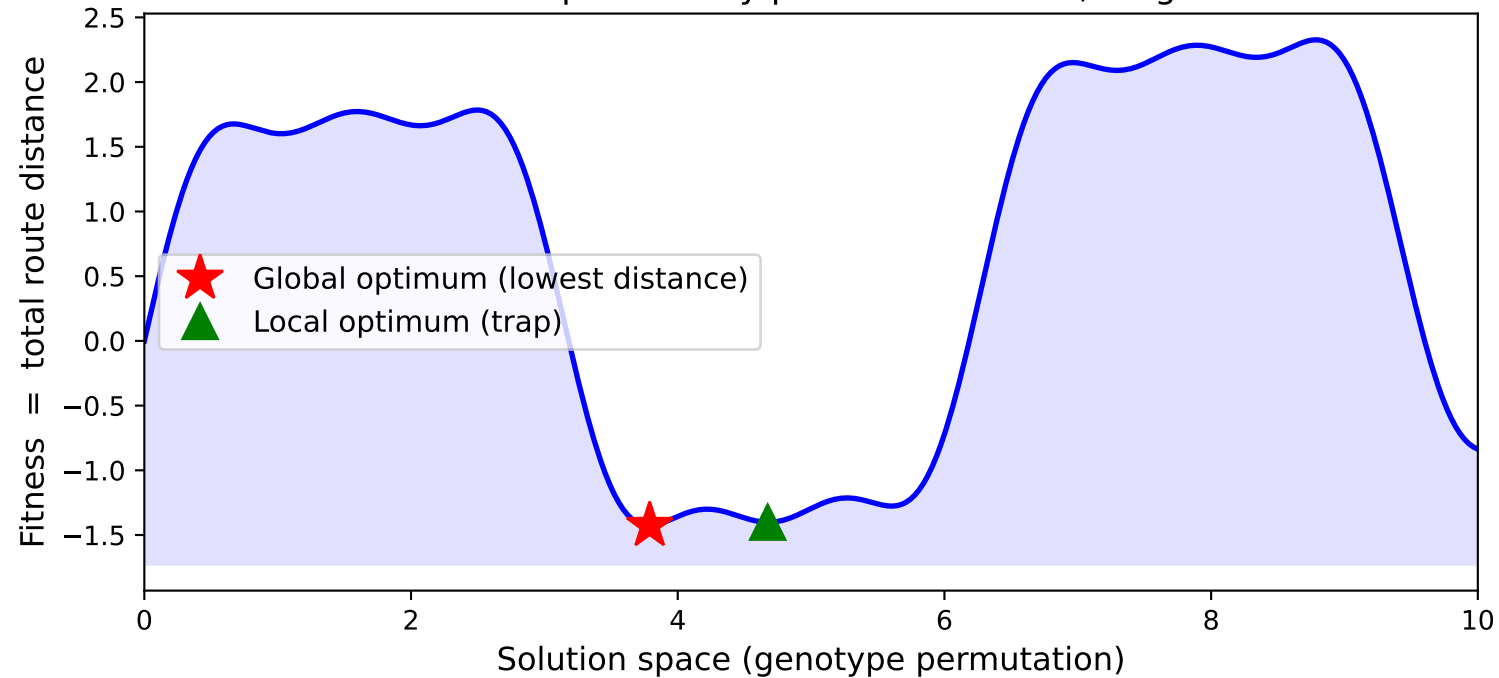
Fitness Landscape — Every point is a solution; height = cost
