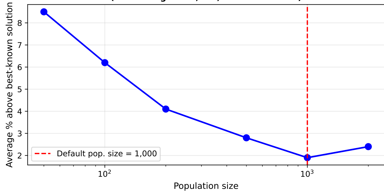
Effect of Population Size (fixed budget = 1,000,000 evaluations)
