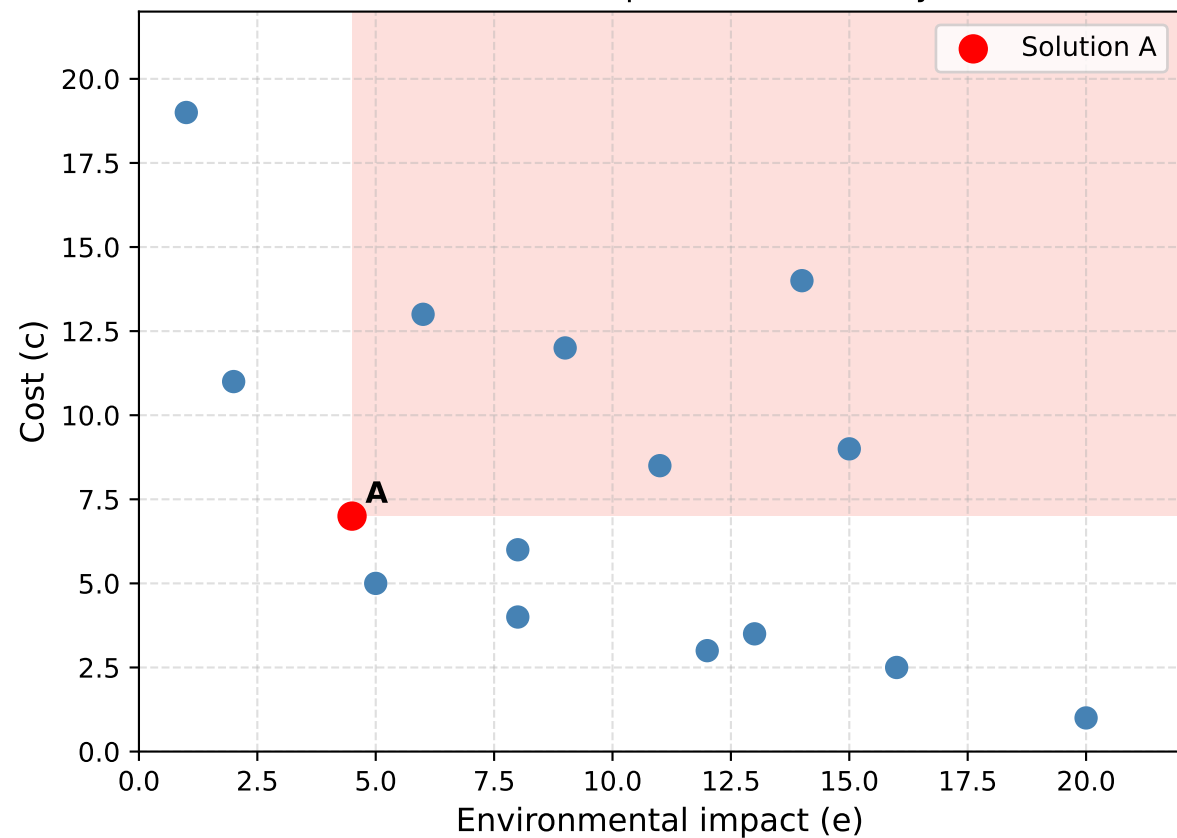
The area of the solution space dominated by solution A
