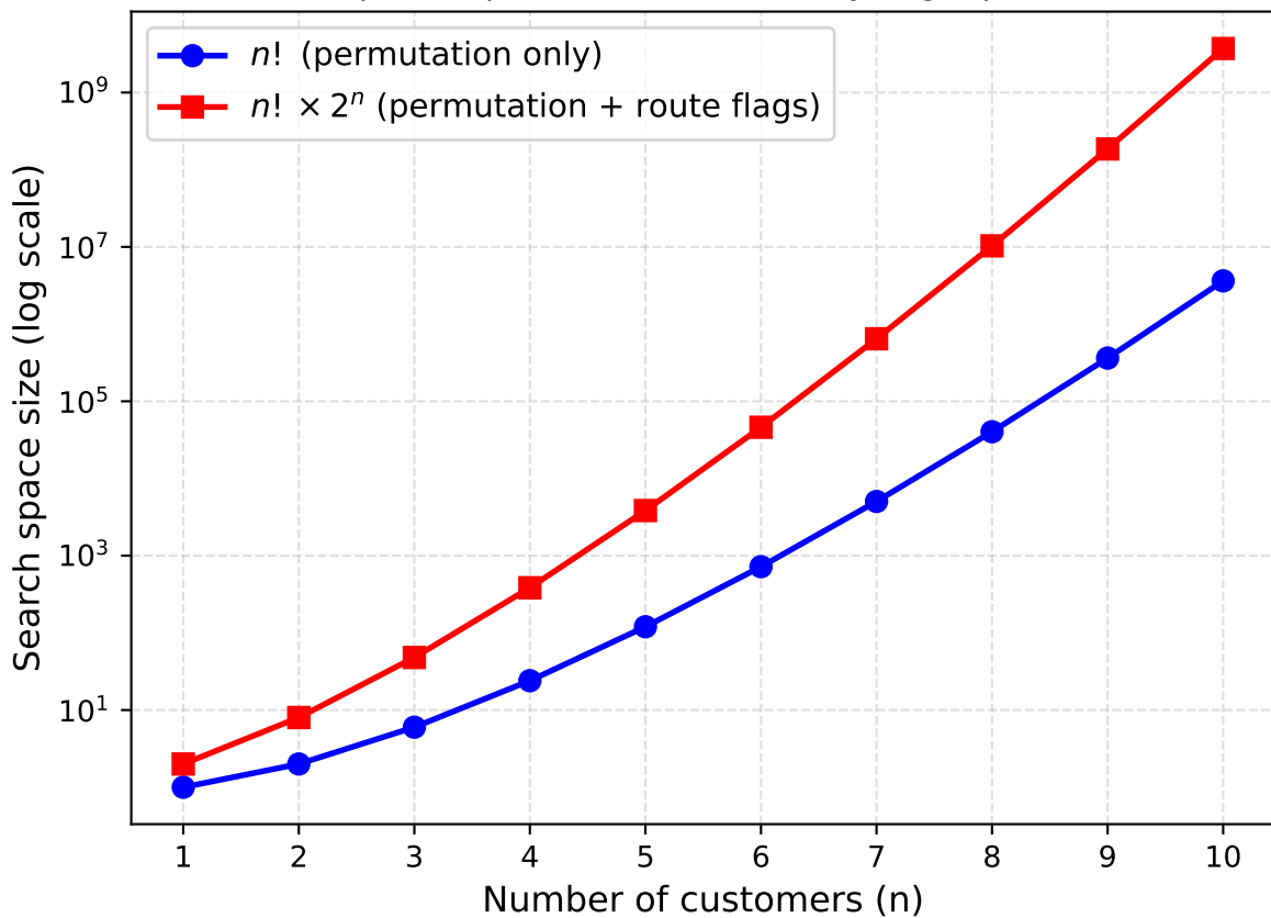
Search space explosion with new binary-flag representation
