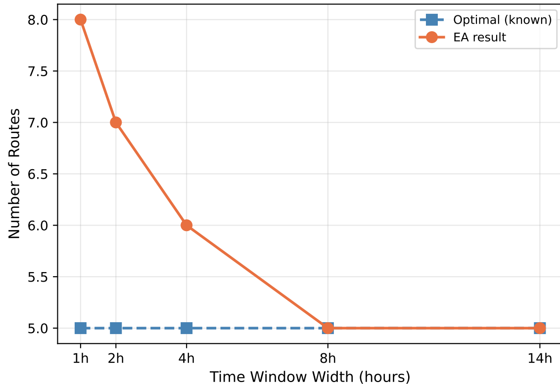
Tighter Time Windows Require More Routes (Benchmark A-n32-k5)
