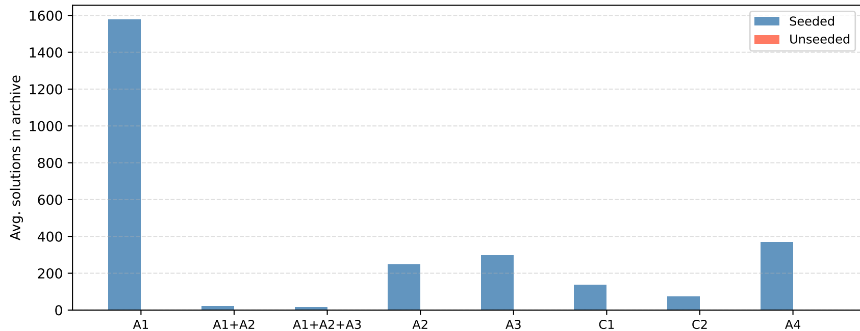
Archive coverage: seeded vs. unseeded MAP-Elites (A problems, Table 6.9 — unseeded archive remains essentially empty)
