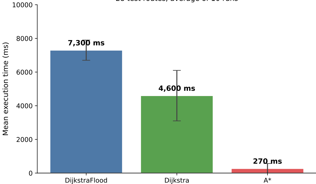
Algorithm Performance -- Edinburgh Graph (63267 nodes) 28 test routes, average of 10 runs
