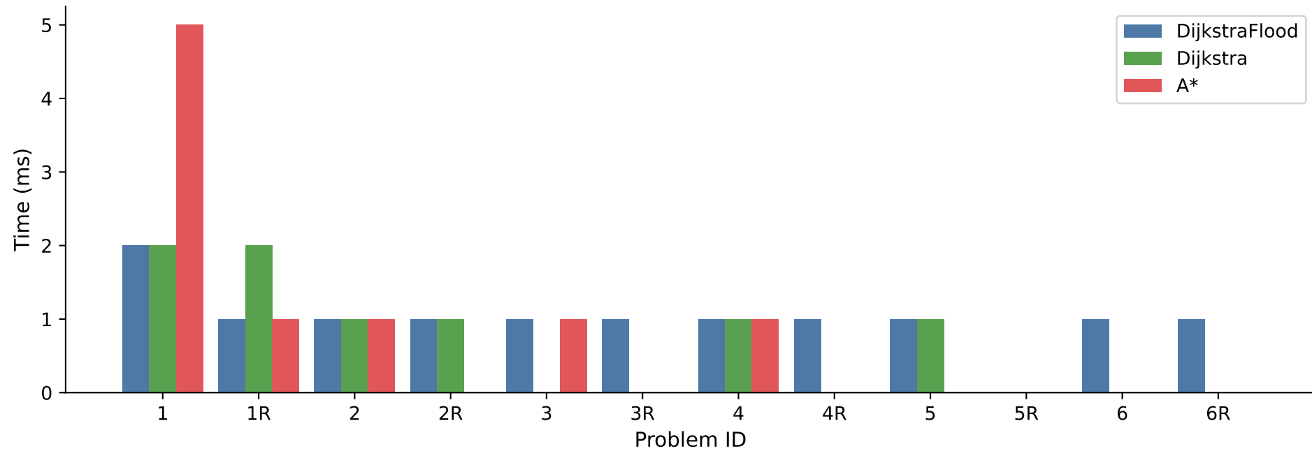
Sirmione Graph (255 nodes) -- Algorithm Execution Times All algorithms find identical distances
