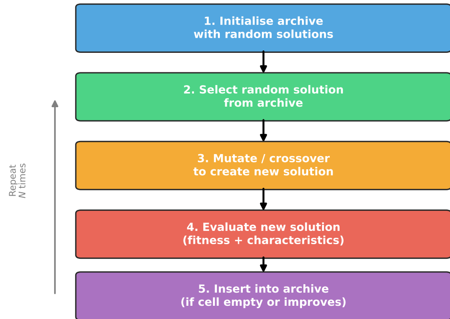
MAP-Elites Algorithm Flow
