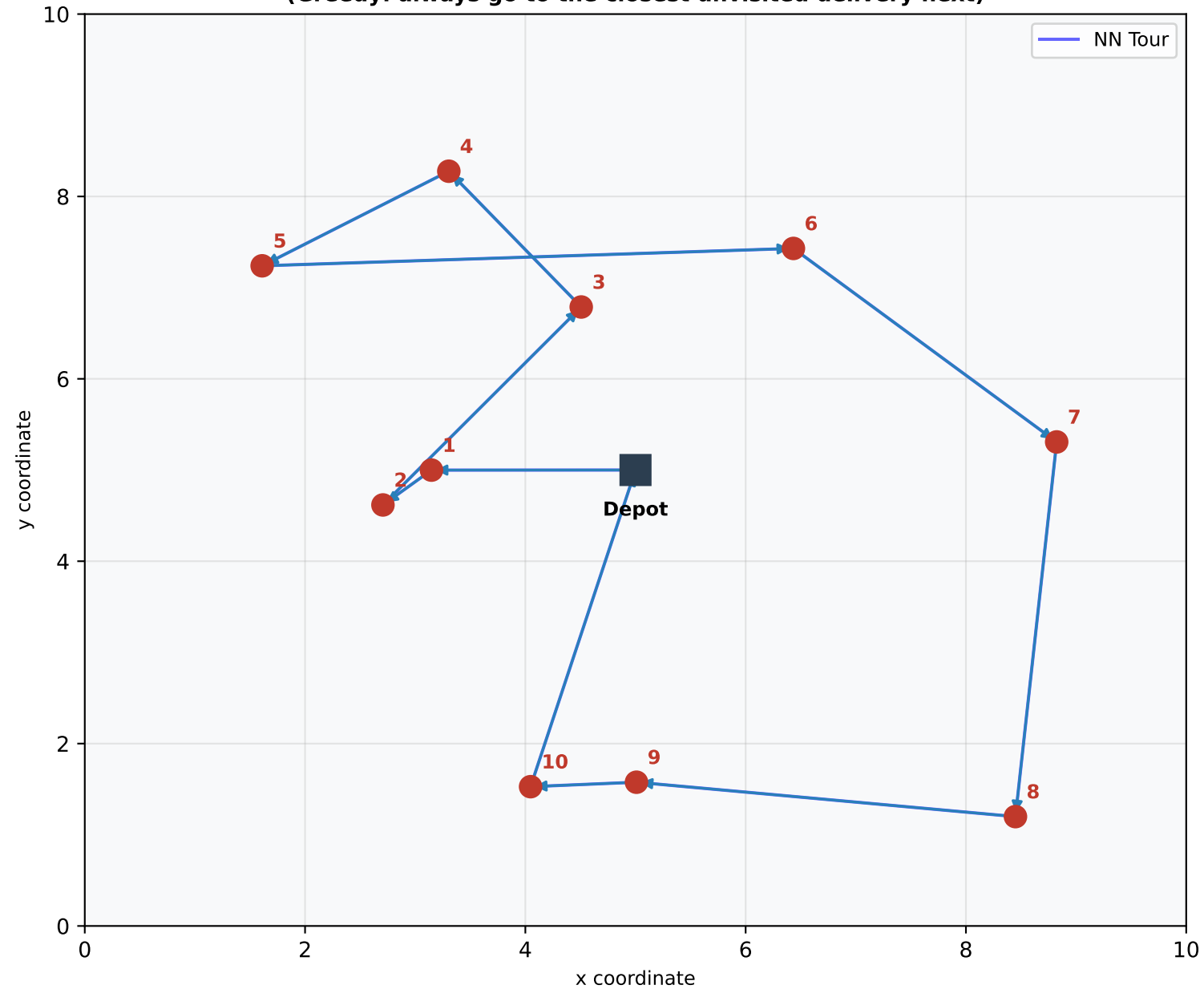
Nearest Neighbour Heuristic for Default Tour Initialisation (Greedy: always go to the closest unvisited delivery next)
