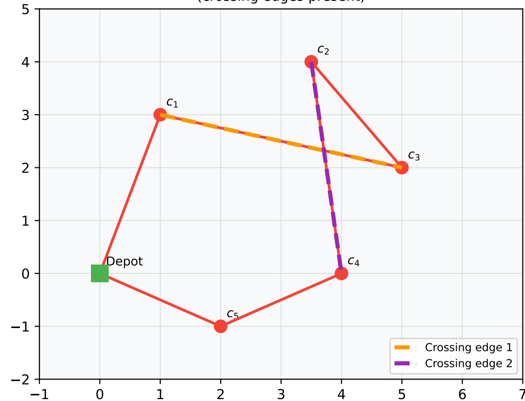
Before 2-opt (crossing edges present)
