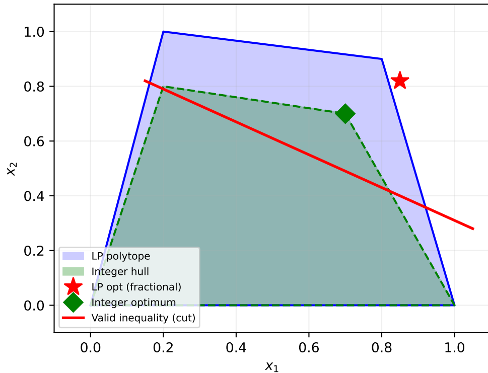
Cutting Plane Tightens LP Feasible Region
