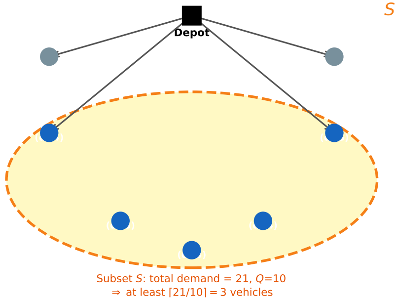
Capacity (Rounded) Cut for customer set S
