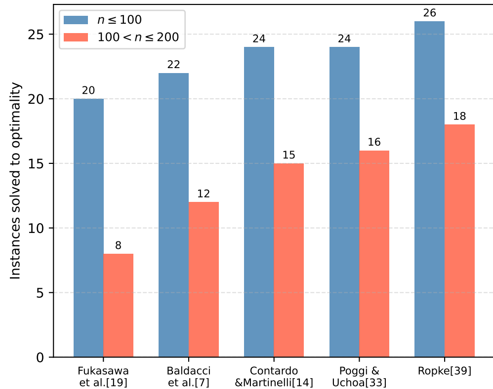
Instances Solved by BPC Algorithm
