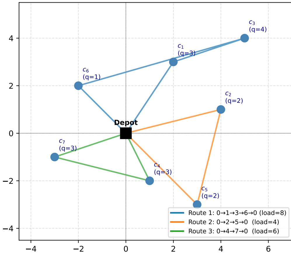
CVRP Instance: Depot, Customers, and Three Routes ( Q = 8 )
