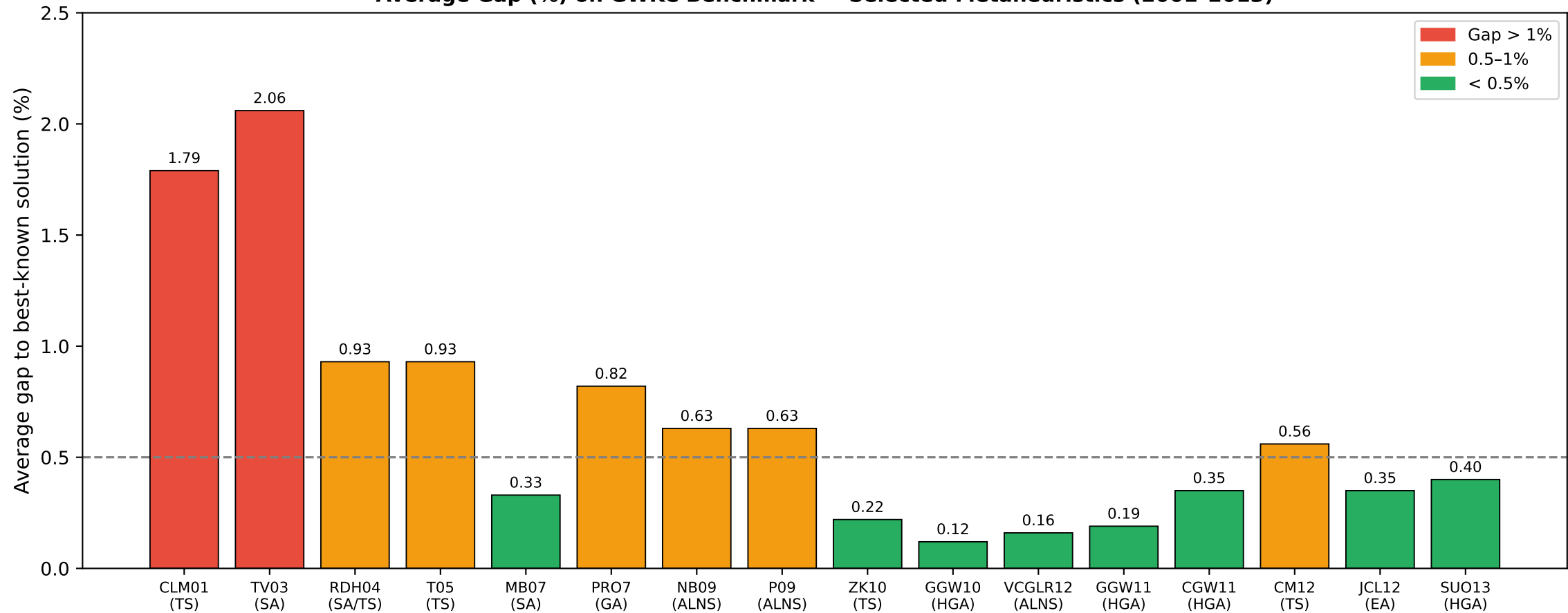
Average Gap (%) on GWKC Benchmark — Selected Metaheuristics (2001-2013)
