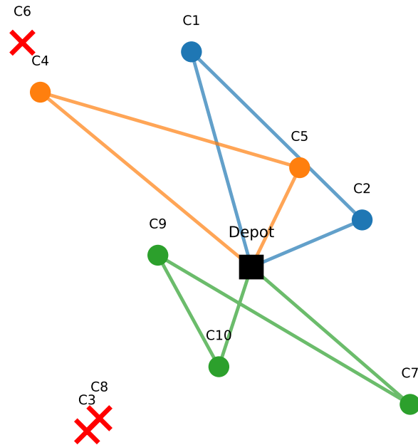
Large Neighbourhood Search (LNS): Destroy Phase (remove customers 3,6,8 shown as red crosses)
