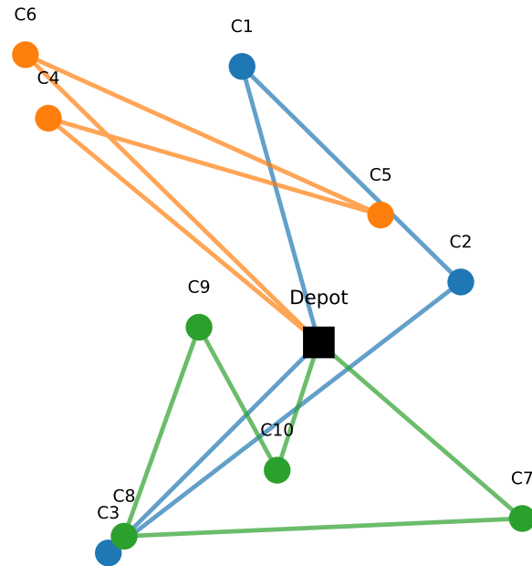
Repair Phase (re-insert removed customers optimally)
