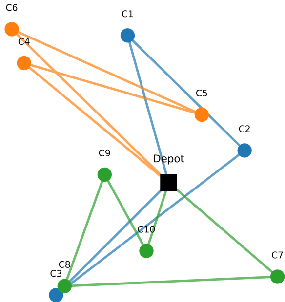
Original Solution (complete routes)
