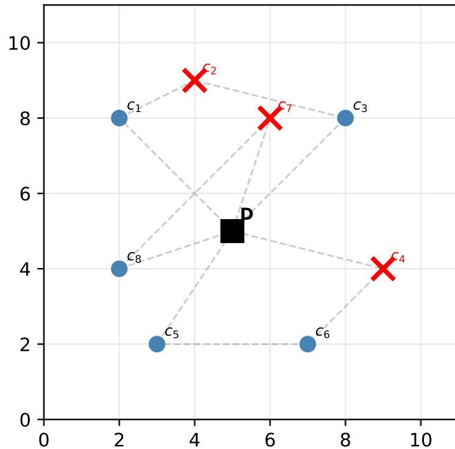
Destroy: Remove 3 random customers
