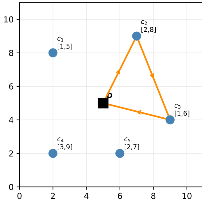
Step 1: Insert cheapest feasible: c_2 between D- c_3
