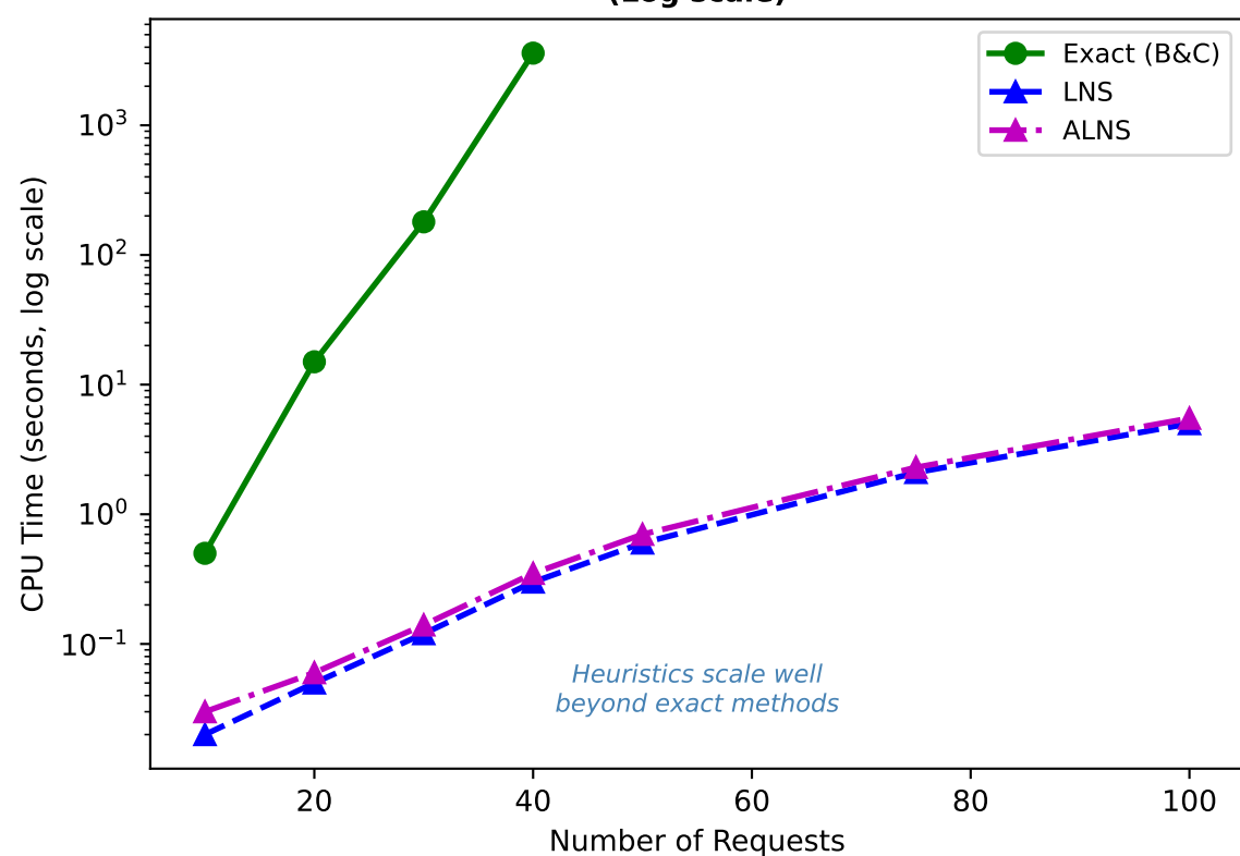
CPU Time vs Instance Size (Log scale)
